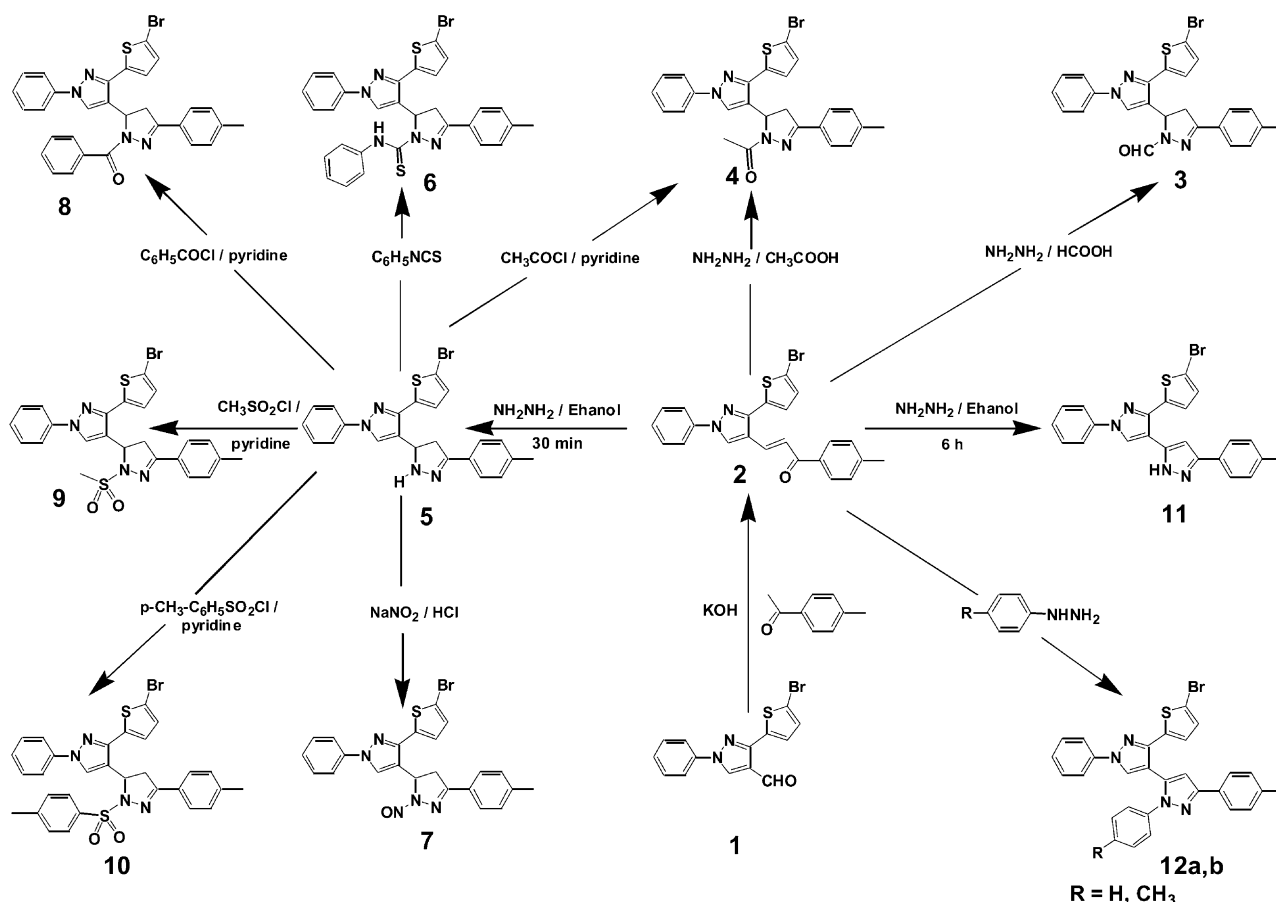
Figure 2. Synthesis of the intermediate and target compounds.
