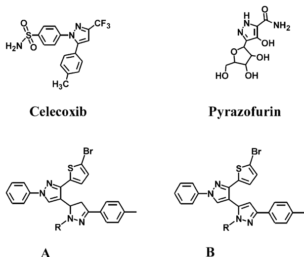
Figure 1. Structures of celecoxib, pyrazofurin and the novel series of pyrazole A and B .
